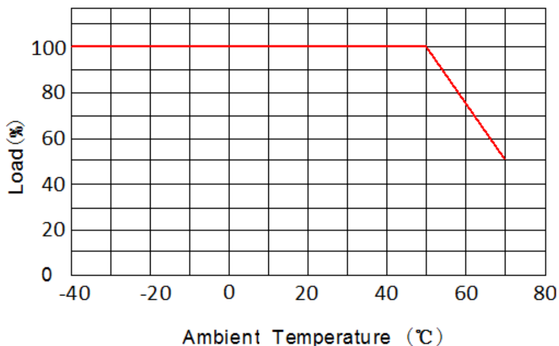
Derating Curve
