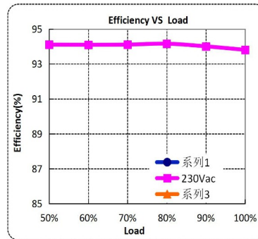
GV6-350B048
