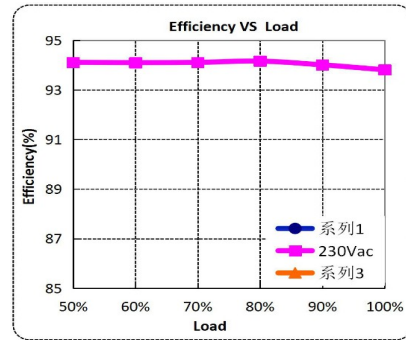
GV6-350B036
