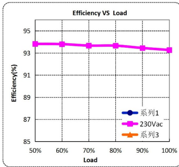
GV6-350B024
